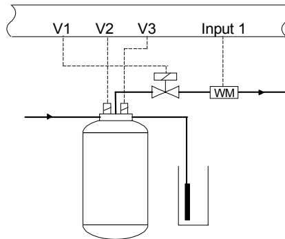
Single filter ion exchanger with EURO valve
