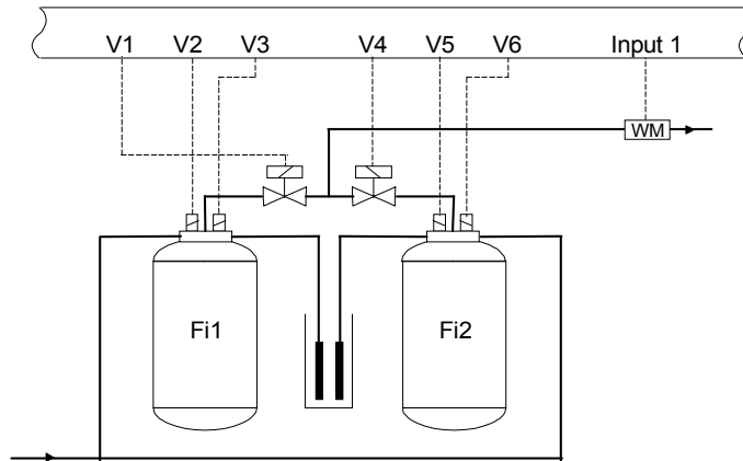
Dual filter ion exchanger with EURO valves.
